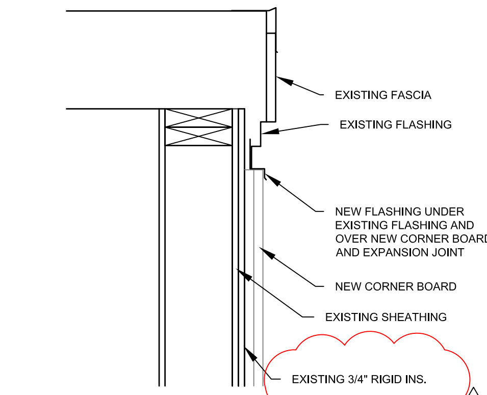
L FLASHING NEW CORNER BOARD IS WIDER THAN EXISTING CORNER BOARD FLASHING AND NEW EXPANSION JOINTS SCALE: 1 1/2" = 1'-0"
