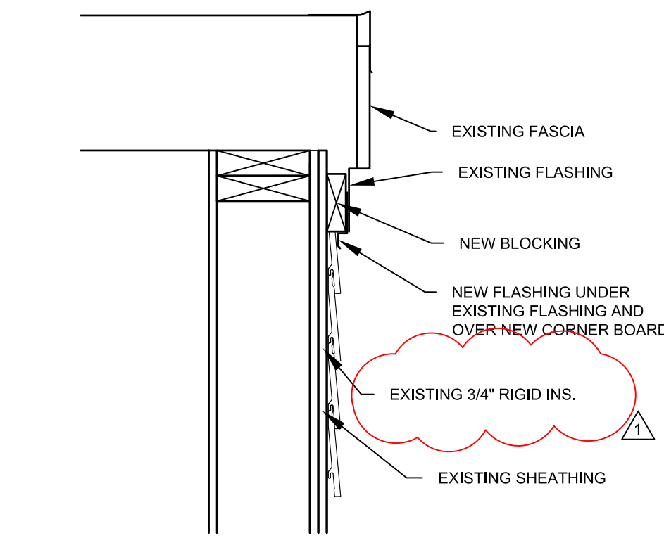
M FLASHING NEW CORNER BOARD IS NARROWER THAN EXISTING CORNER BOARD FLASHING SCALE: 1 1/2" = 1'-0"
