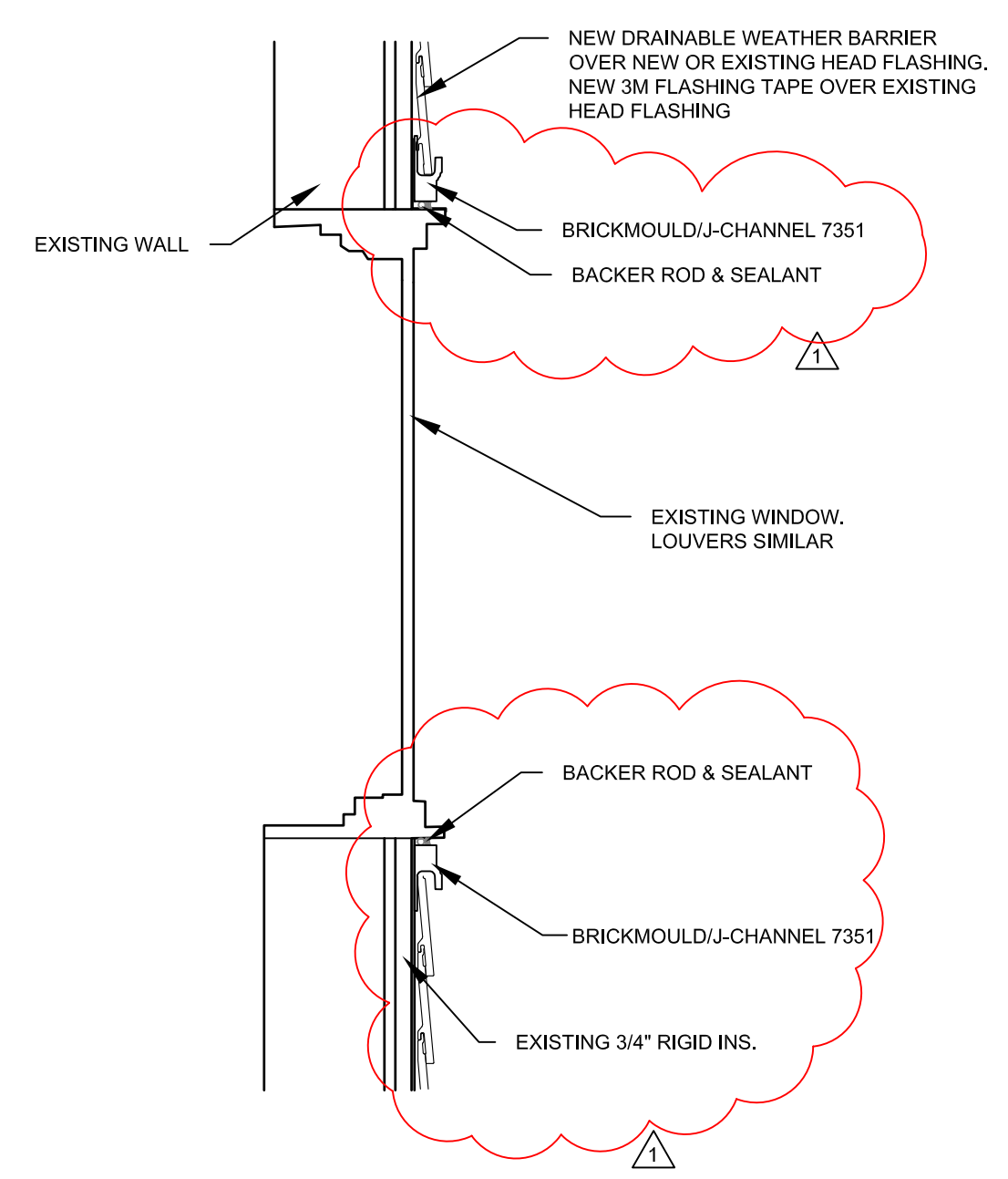
OPENING TRIM DETAIL SCALE: 1 1/2" = 1'-0"
