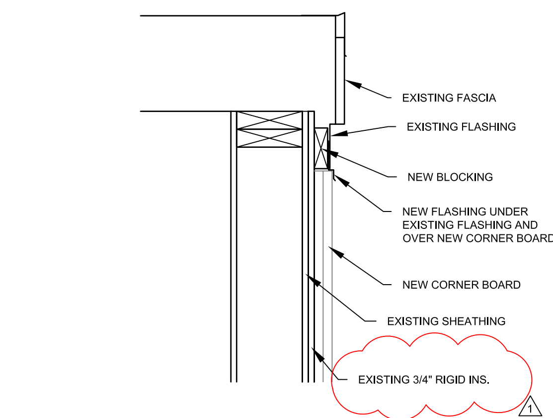
K FLASHING CORNER BOARD ABUTTING EXISTING CORNER BOARD FLASHING SCALE: 1 1/2" = 1'-0"
