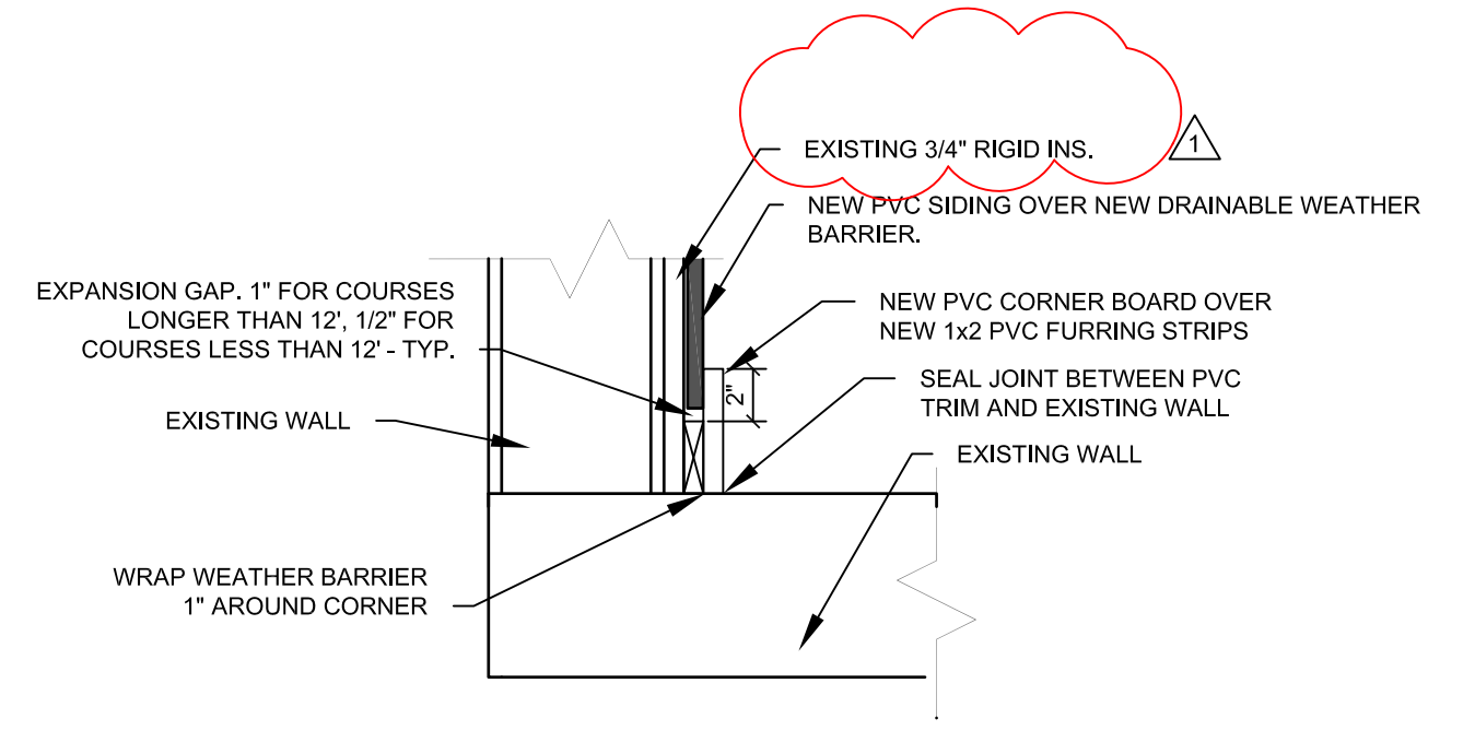
CORNER BOARD DETAIL SCALE: 1 1/2" = 1'-0"
